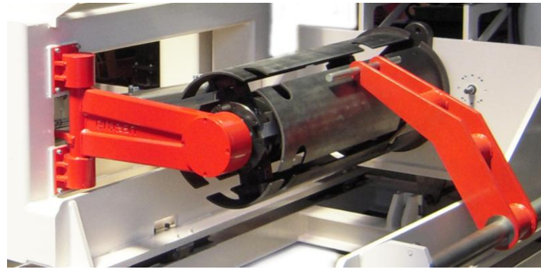
Expanding mandrels are made in house, to suit the exact requirement of the machine and product to be made.
