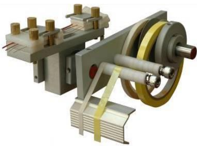
Multi-wire feeder head with margin taping
