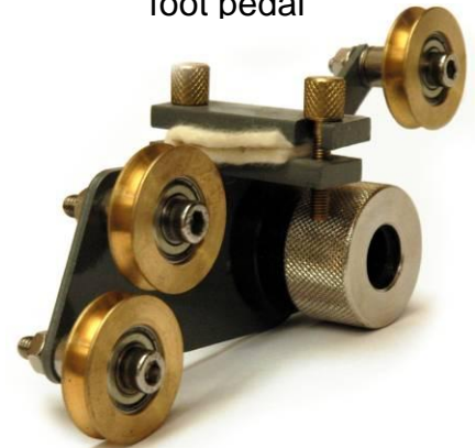
Roller feeder
